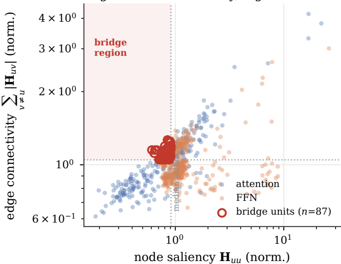
Bridge units: low saliency, high connectivity
